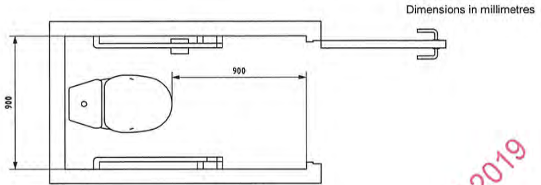
Figure 35 — Ambulant toilet
