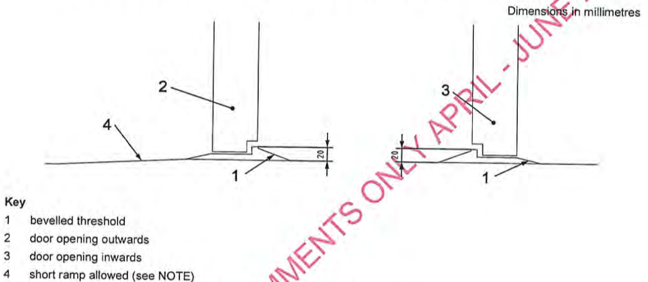
Figure 10 — Bevelled threshold
