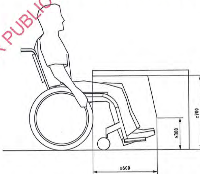
Figure 61 — Table and desk height for wheelchair users
