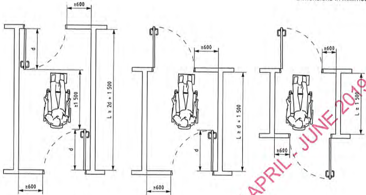
Figure 12 — Minimum dimensions of lobbies with single leaf single swing doors
