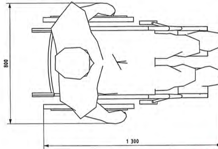
Figure B.1 — Footprint of a wheelchair user
