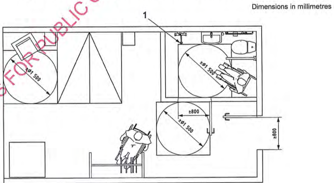
Figure 50 — Example of space allowances for accessible bedroom
