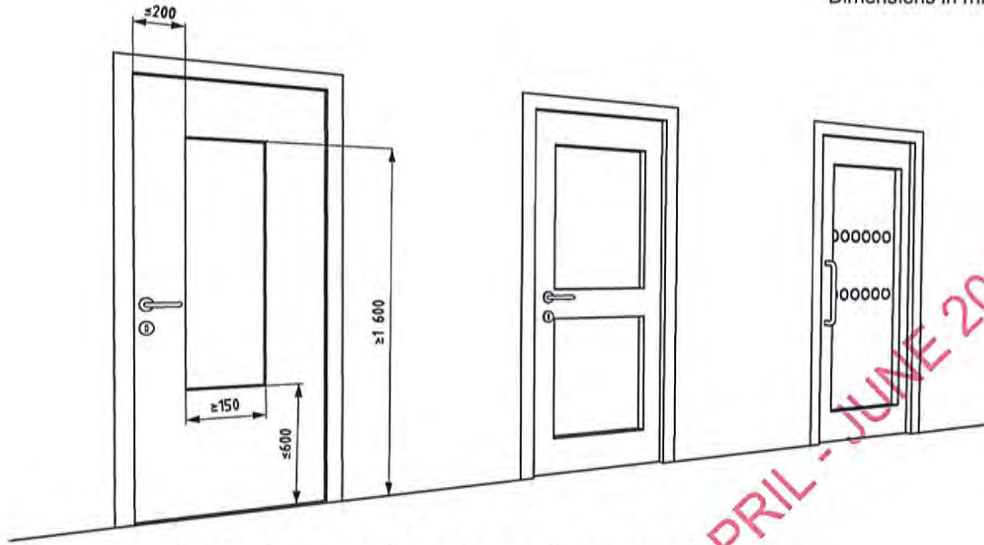
Figure 28 — Examples of doors with glazed viewing panels
