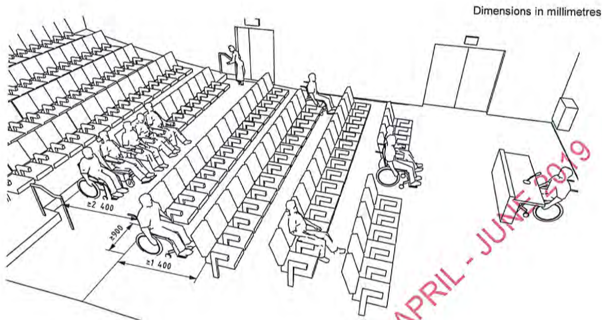
Figure 34 — Examples of viewing spaces for wheelchair users
